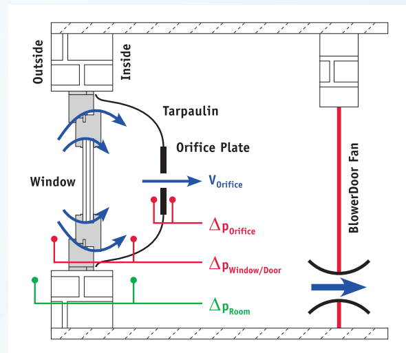
Principle for the determination of the joint permeability of windows
