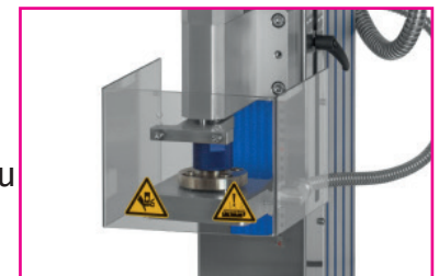
sealing head with heat protection shield
