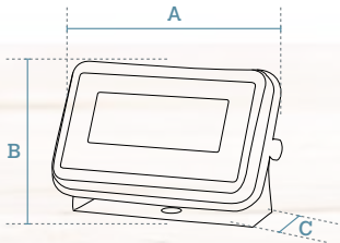
Dimensions DATA IN mm
