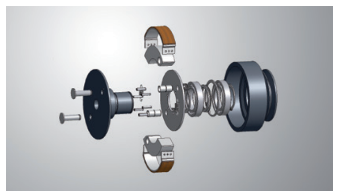
Exploded view of the turning jaw execution
