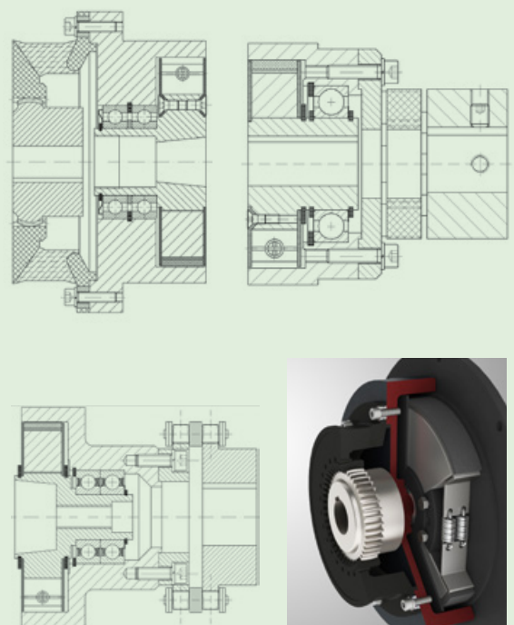
Centrifugal clutch combined with highly flexible clutch
