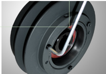
Centrifugal clutch with mechanical belt tensioner
