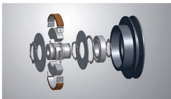
Exploded view of the dovetail execution
