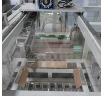
Loading Position
