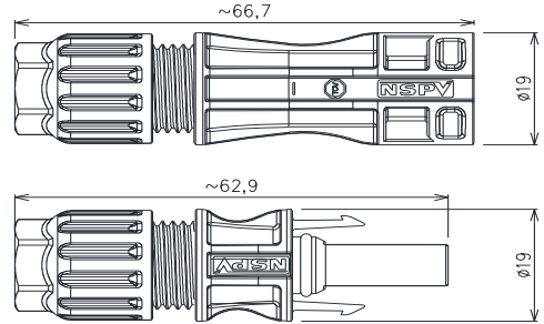
Newsun 1500VDC cable connector:
