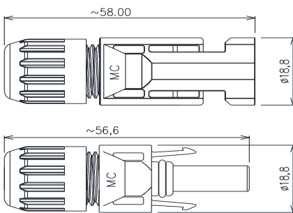
MC4 cable connector
