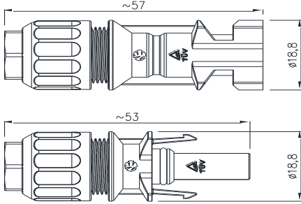
Newsun 1000VDC cable connector:
