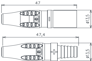
Newsun 1000VDC PV3.0 cable connector:
