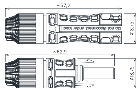
MC4_EVO cable connector
