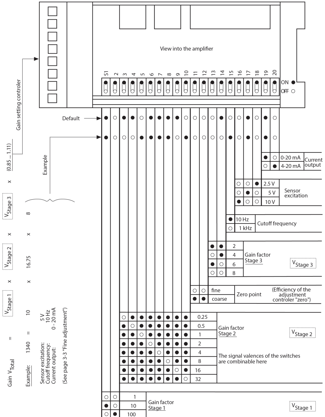
Figure 1: DIP switches of the mounting rail version
